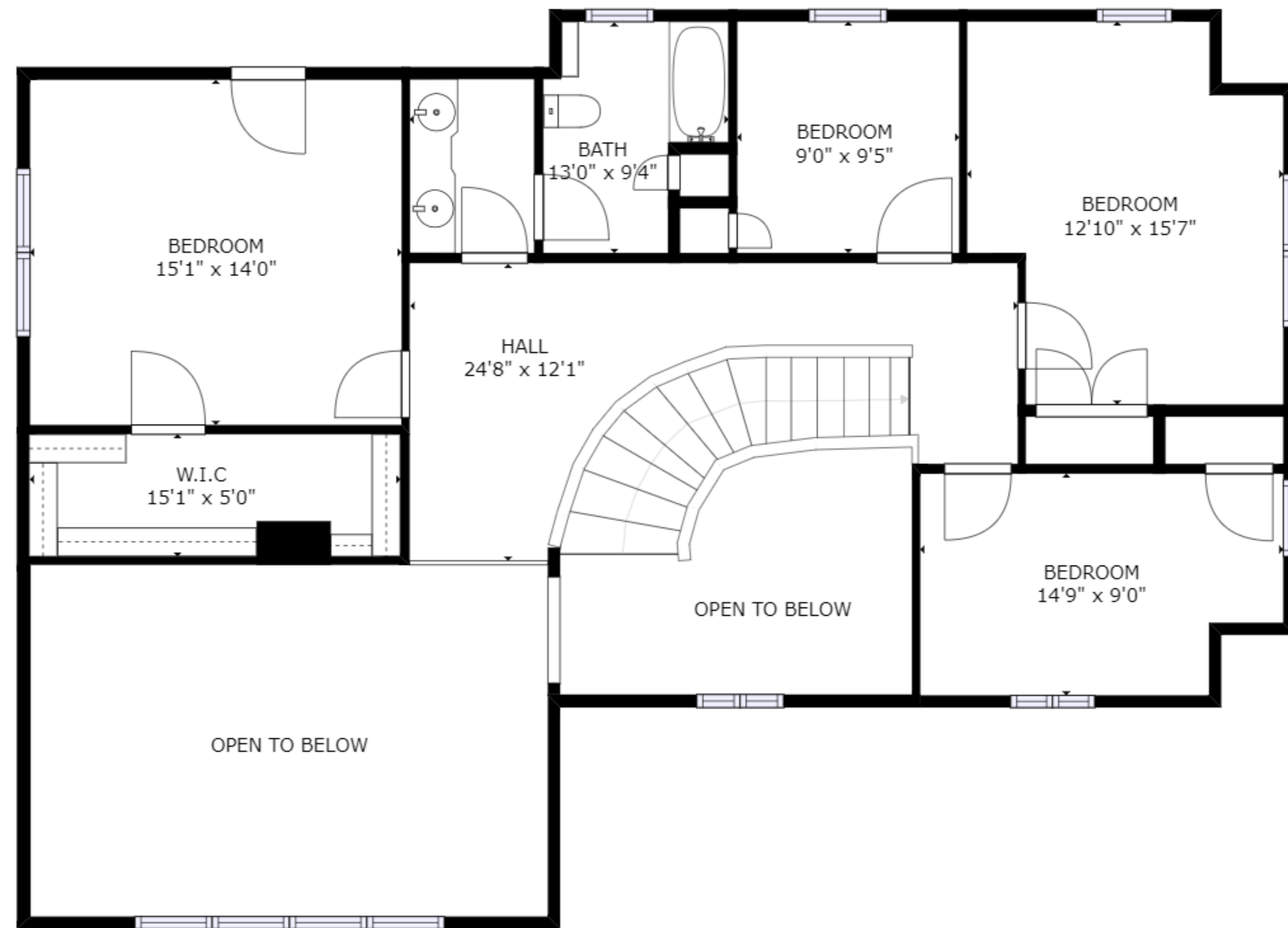
FLOOR 2
