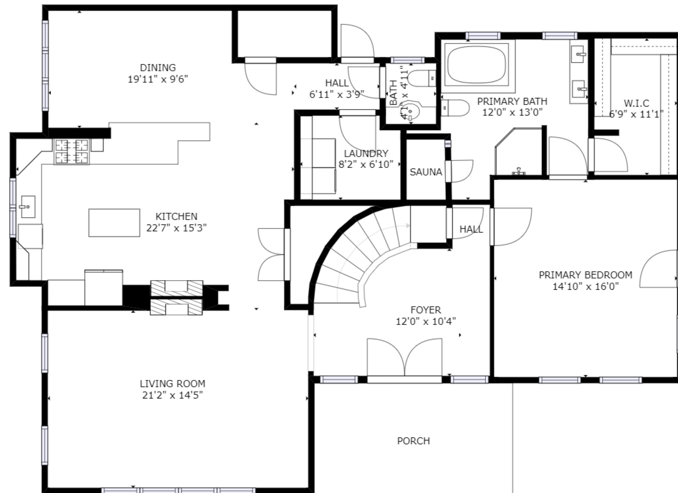
FLOOR 2
